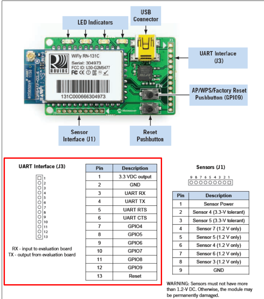
FIGURE 1-2: RN131 EVALUATION BOARD COMPONENTS
